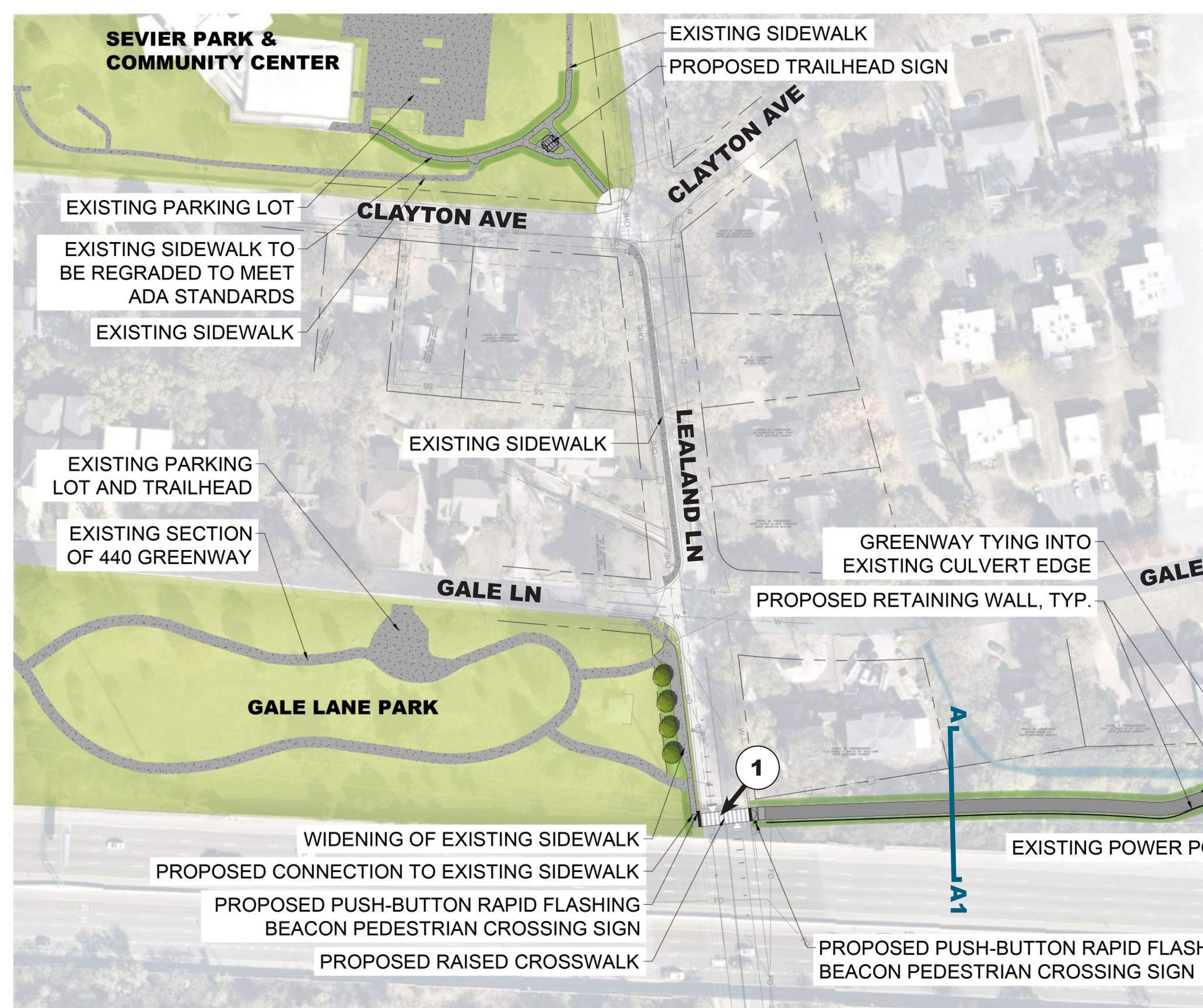
1 LEALAND LANE RAISED PEDESTRIAN CROSSING
